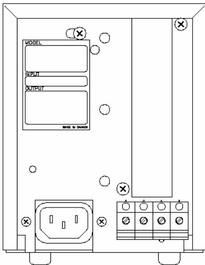
Figure 1. Rear Panel of XT Series Power Supply and 60V HPD Connection designations on the terminal block from left to right are: -Sns, -, +, +Sns
